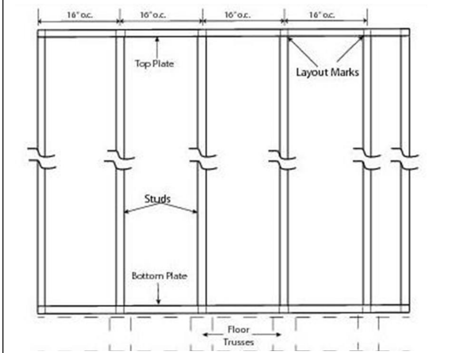
Figure 6.13 - Plate Layout
