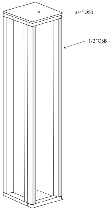
Figure 6.22 – Chases
