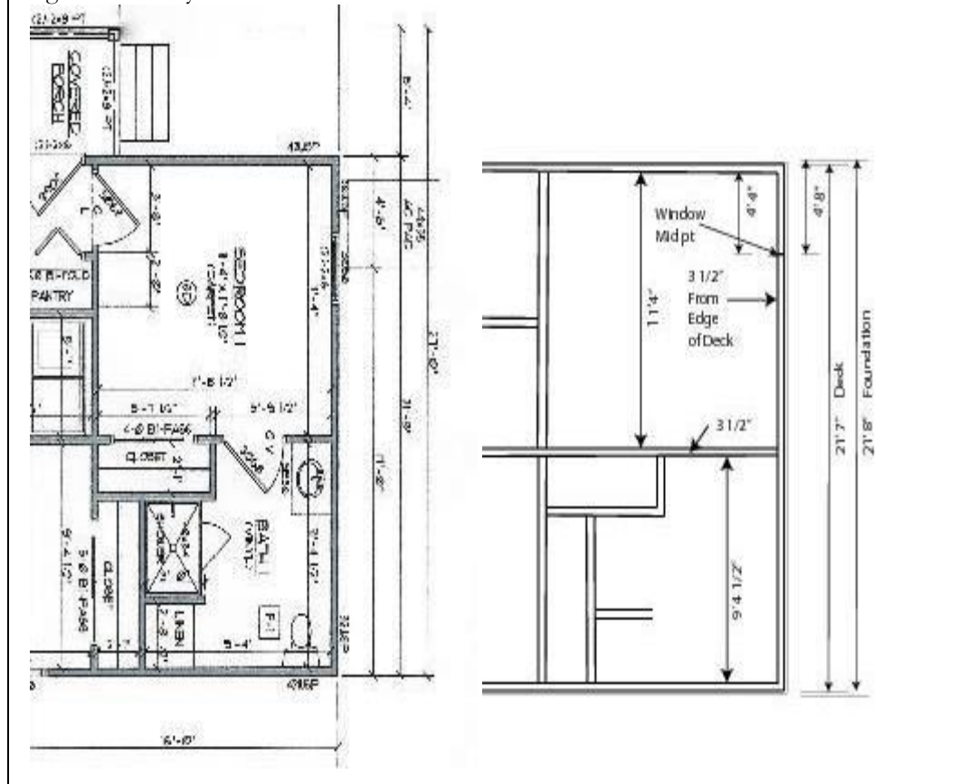
Figure 6.10 – Layout walls on the Deck
