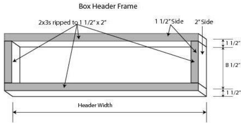
Figure 6.2 – Box Header
